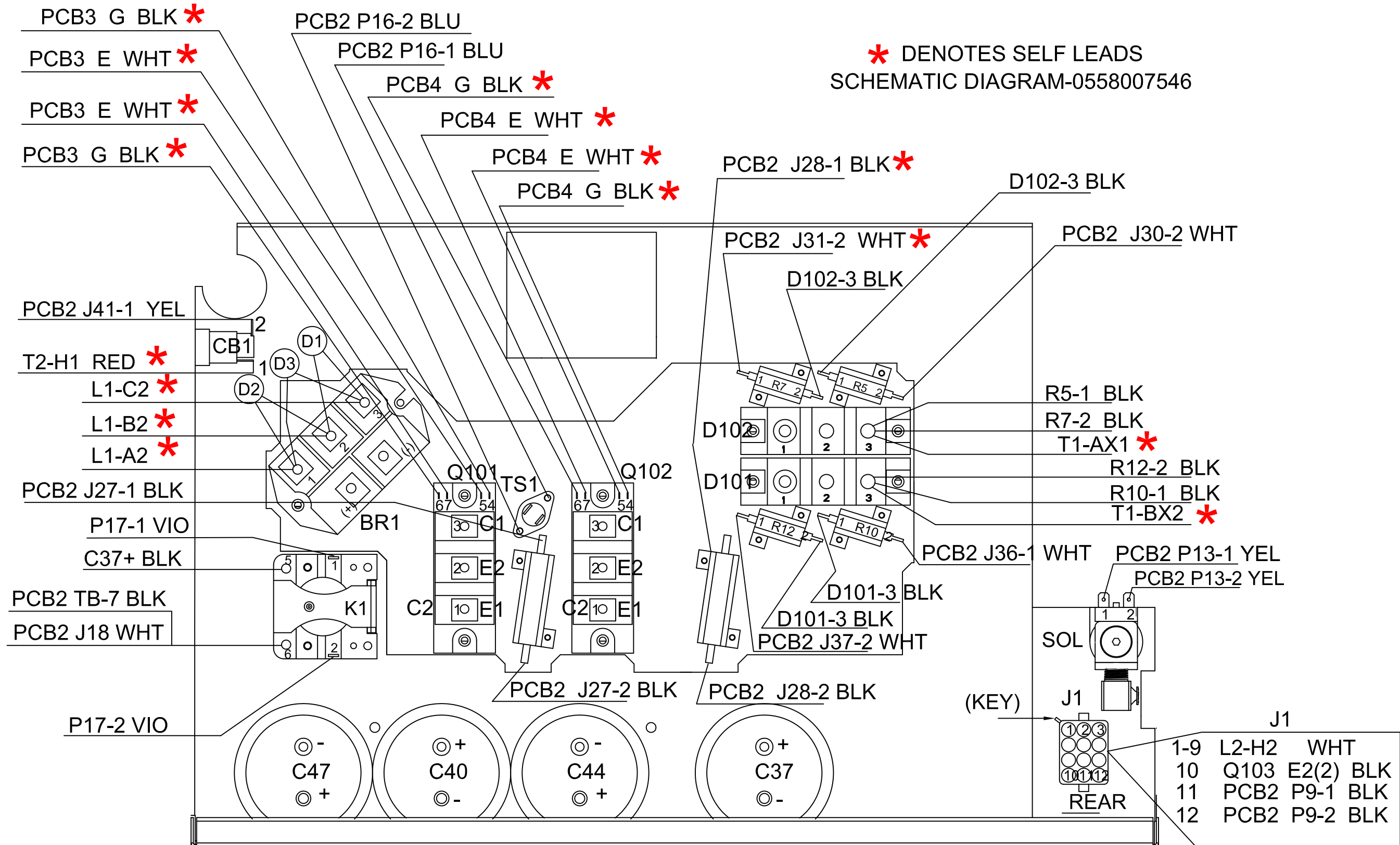
5.2 Wiring Diagram 400/400V CE (0558007547)
