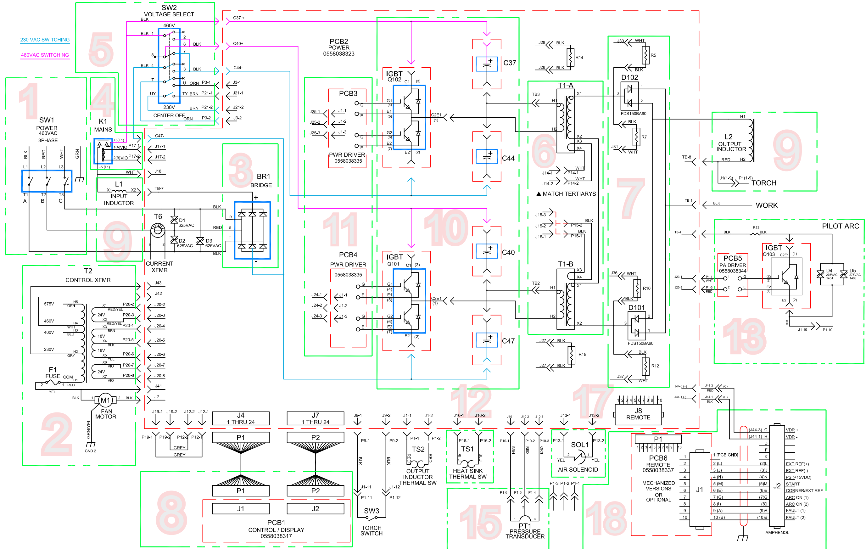
4.0 Schematic Section Map 230/460V- 0558007542
