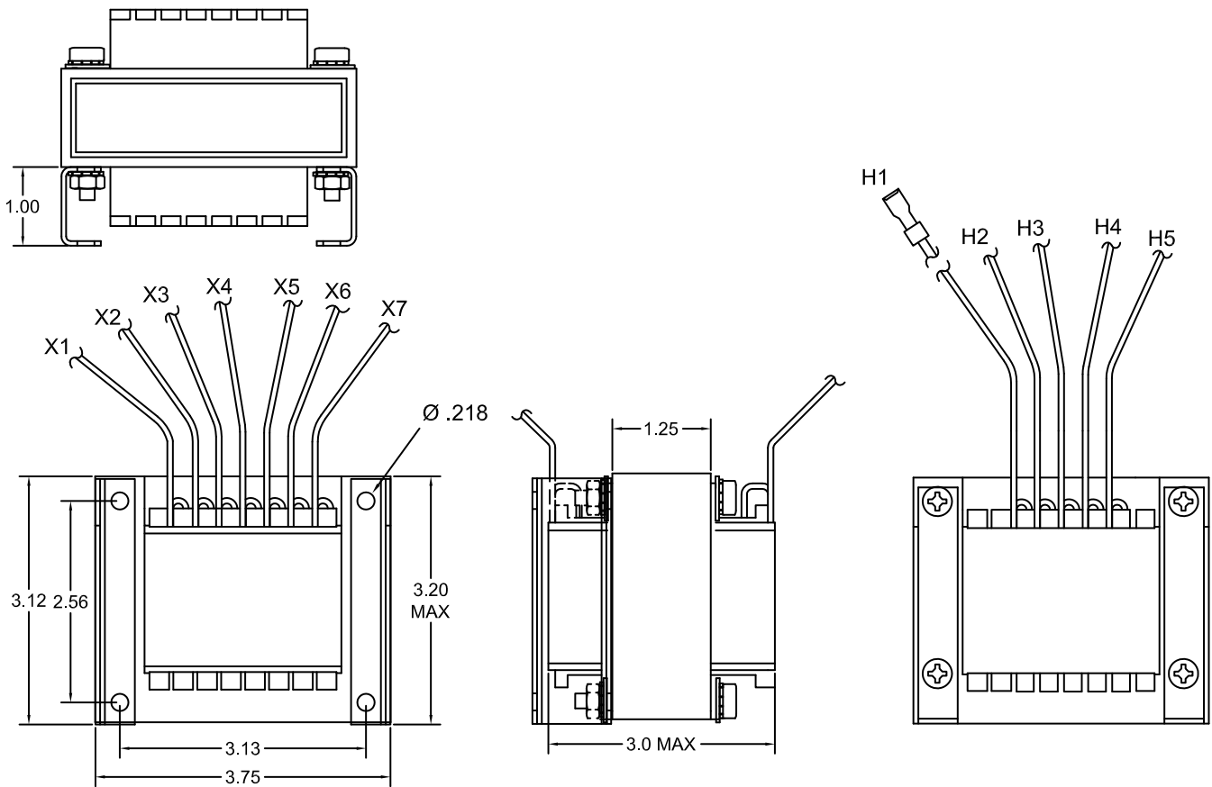
Control Transformer T2 Layout (0558007188)
