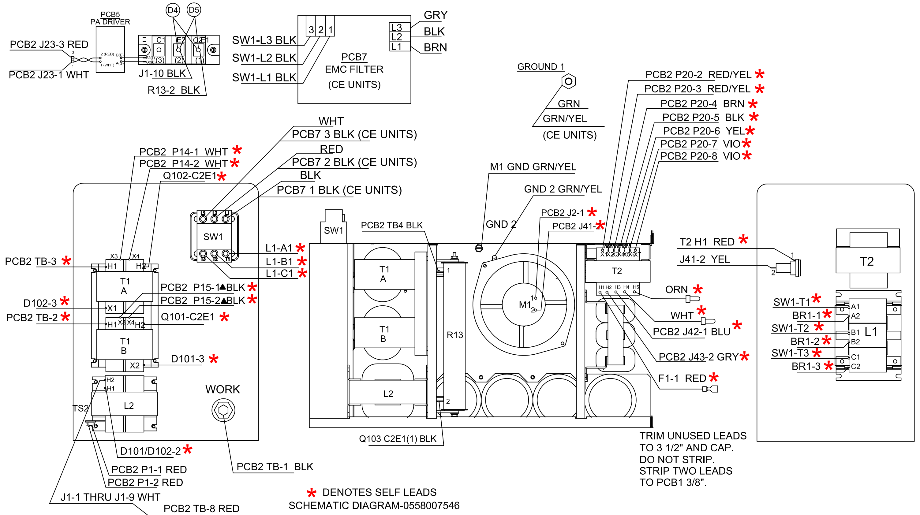
5.2 Wiring Diagram 400/400V CE (0558007547)
