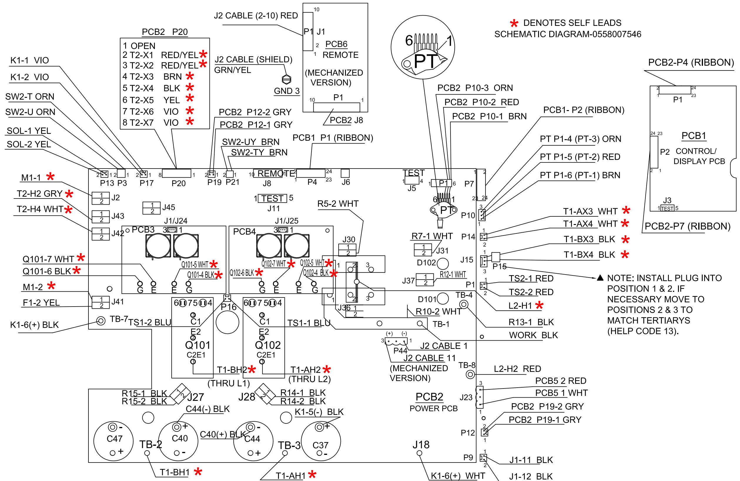
5.2 Wiring Diagram 400/400V CE (0558007547)
