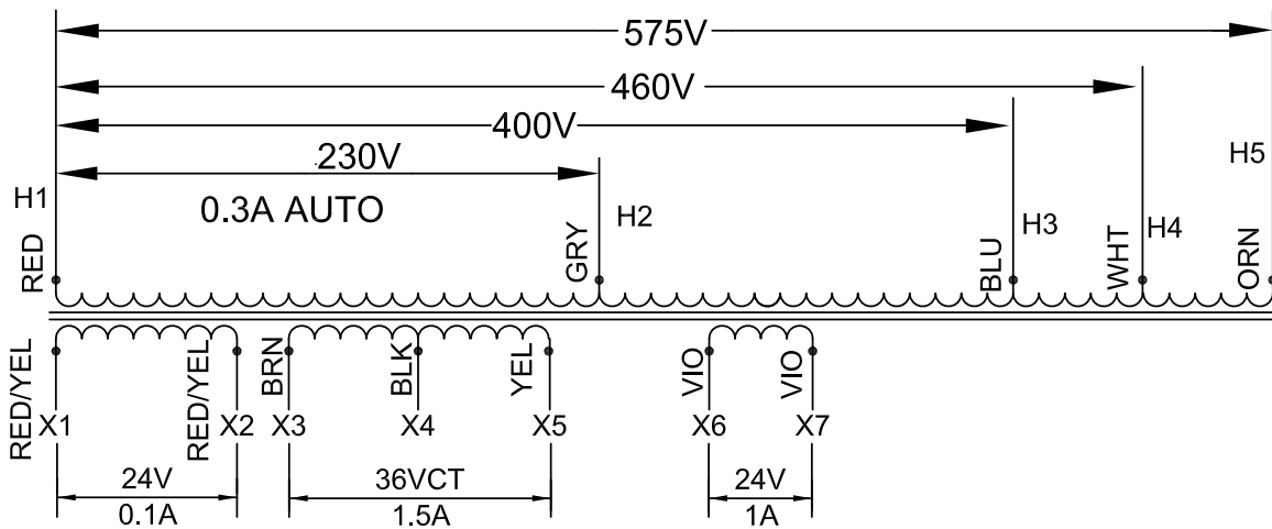
SCHEMATIC DIAGRAM
