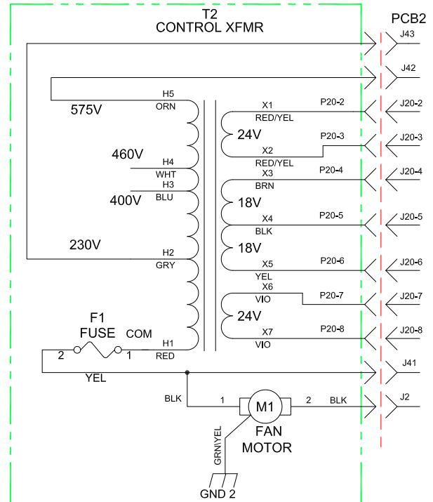
575 V Configuration
