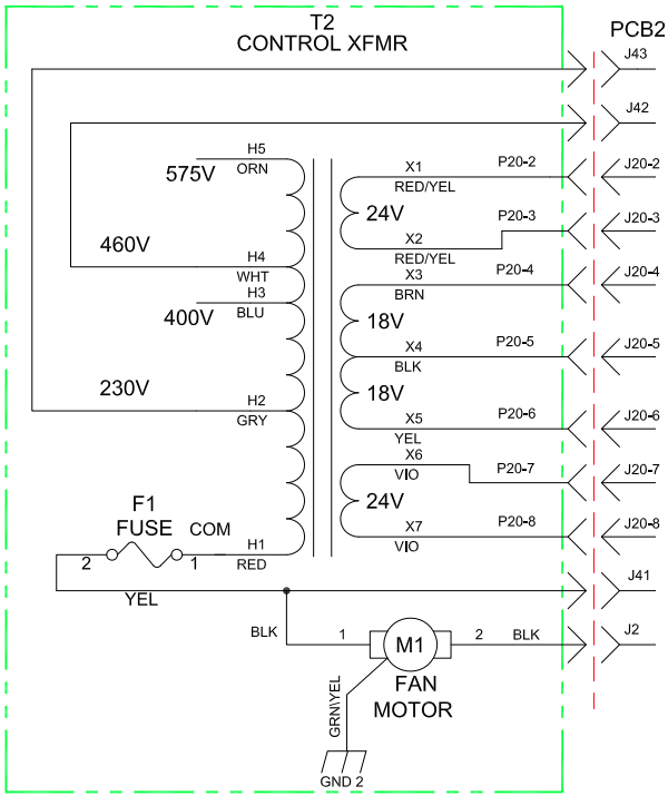
230 V / 460 V Configuration
