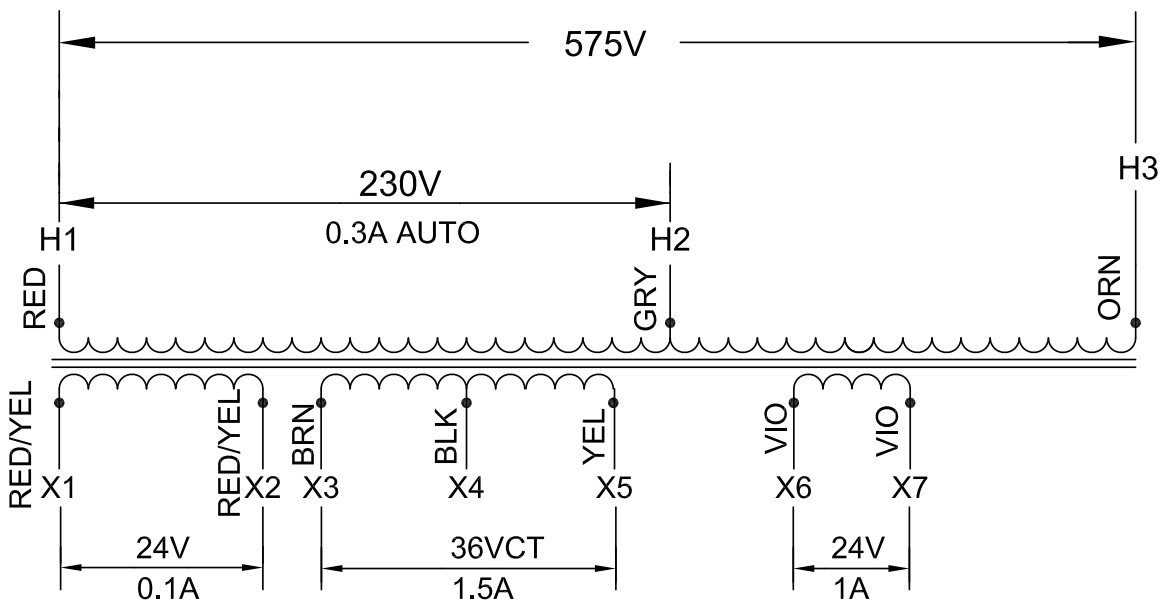
SCHEMATIC DIAGRAM
