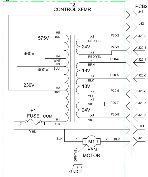
400 V / 400 V CE Configuration
